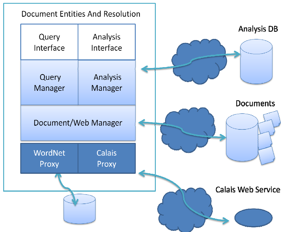
Figure 1: DEAR architecture and related resources
